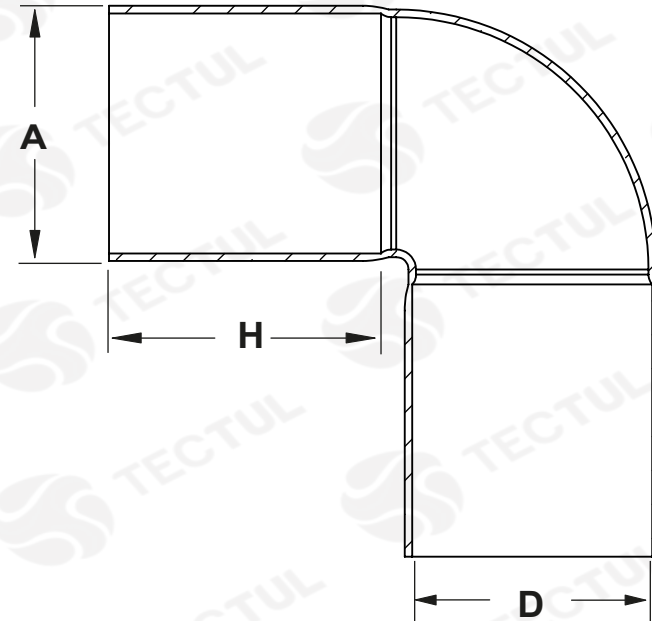
* Informational type cross section view. It does not represent a specific version of the copper fitting.
